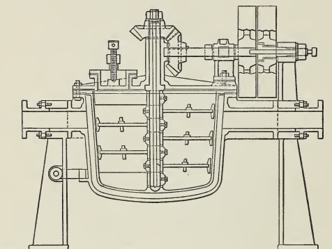
FIG. 11a.—Zemsch's Steam-jacketed Melting and Cooking Kettle.
